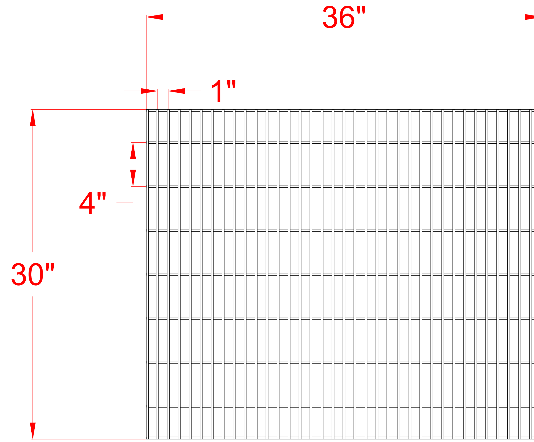
TOP VIEW
