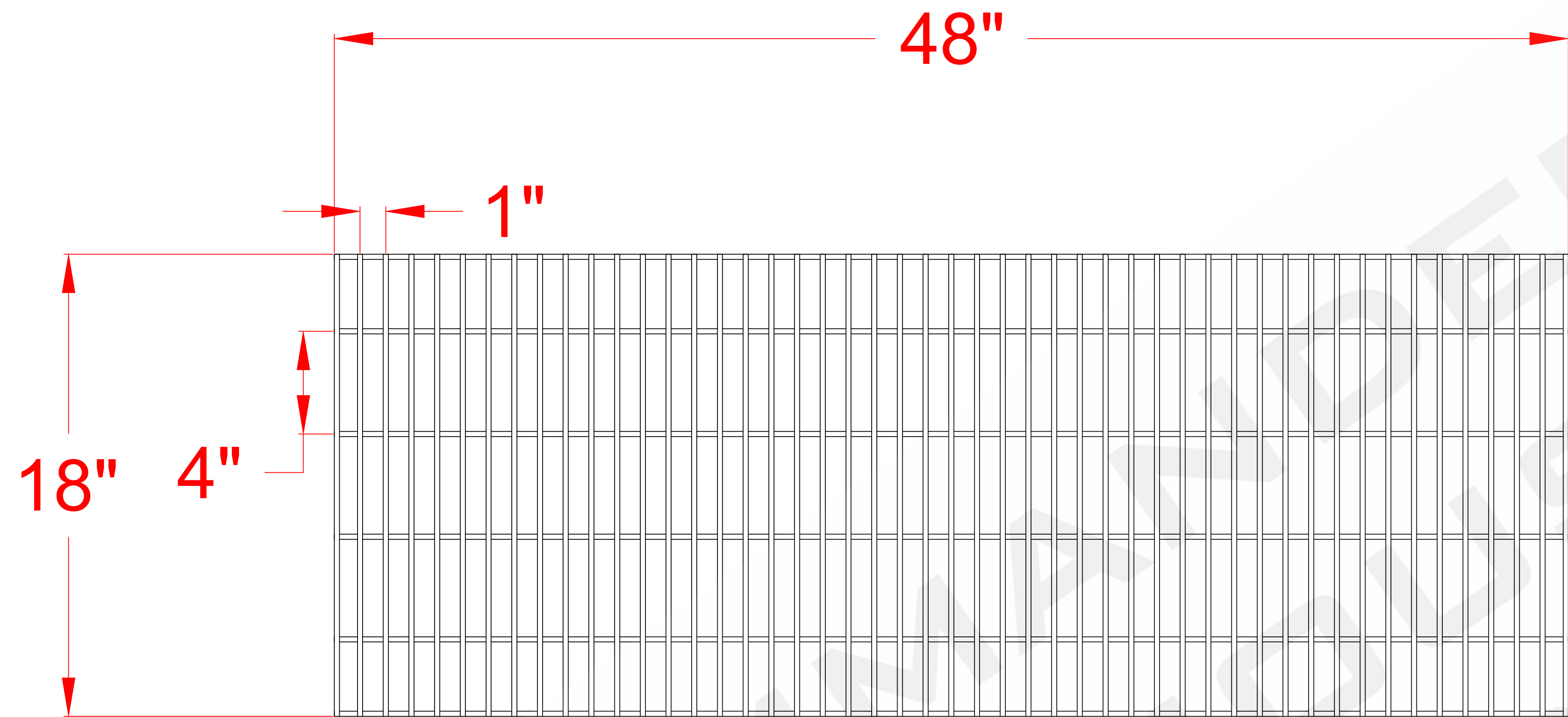
TOP VIEW
