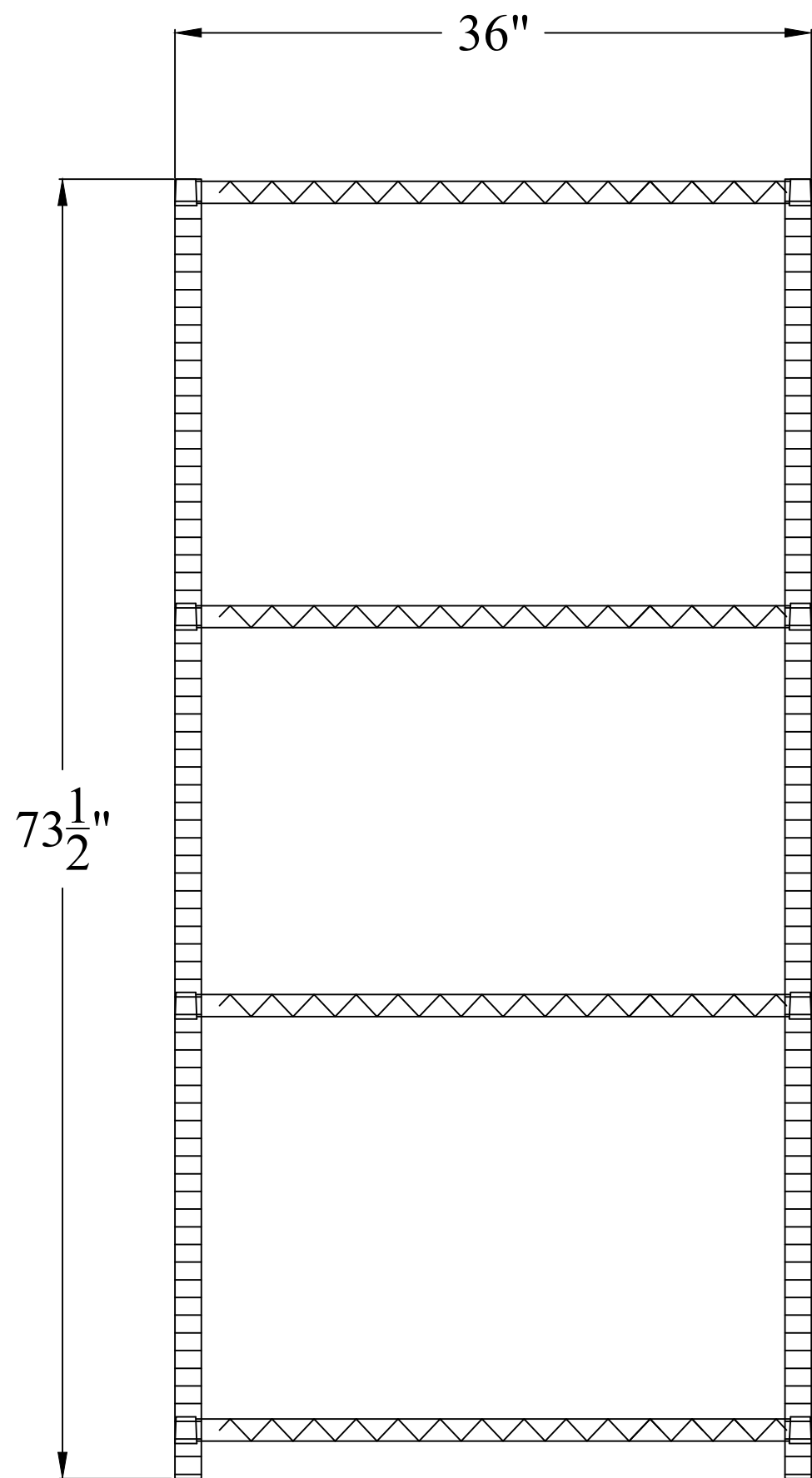
FRONT VIEW
