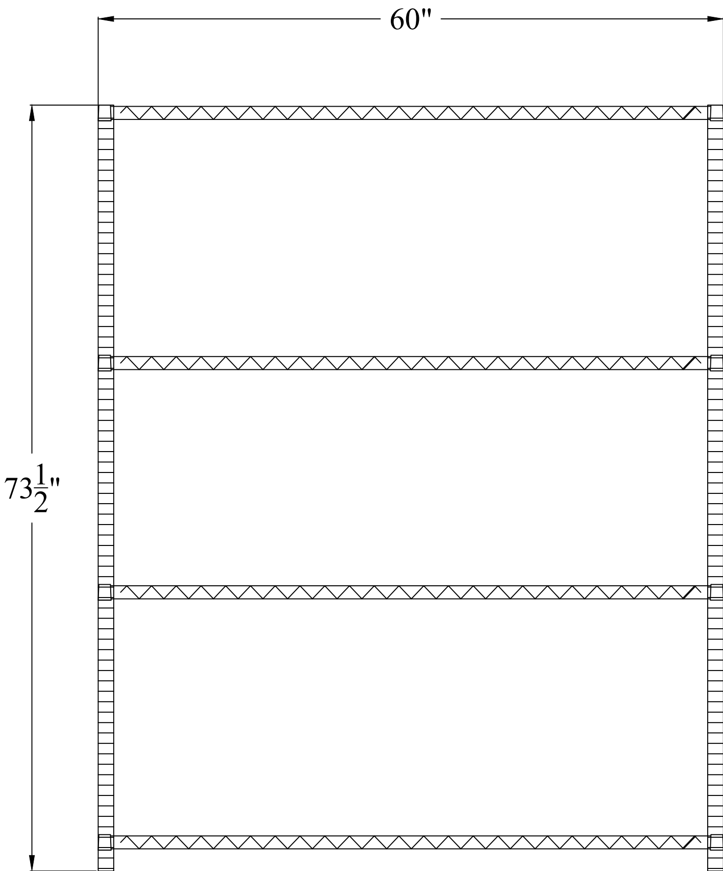
FRONT VIEW
