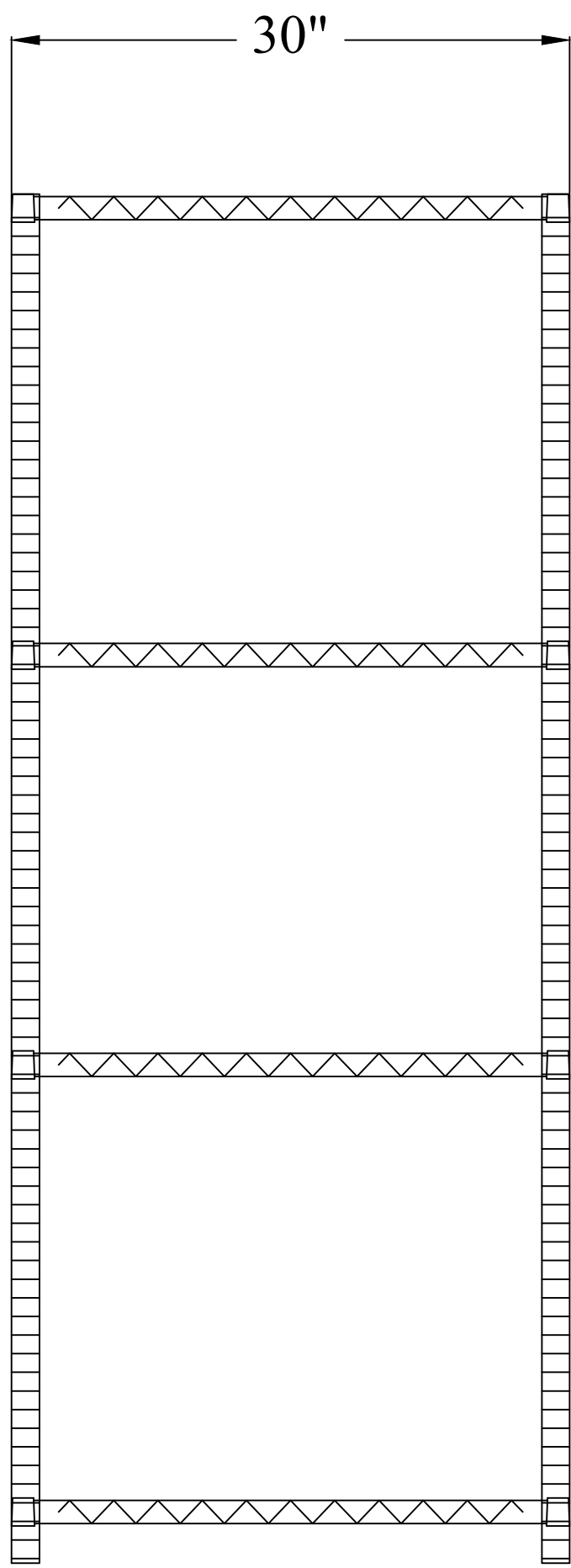
SIDE VIEW
