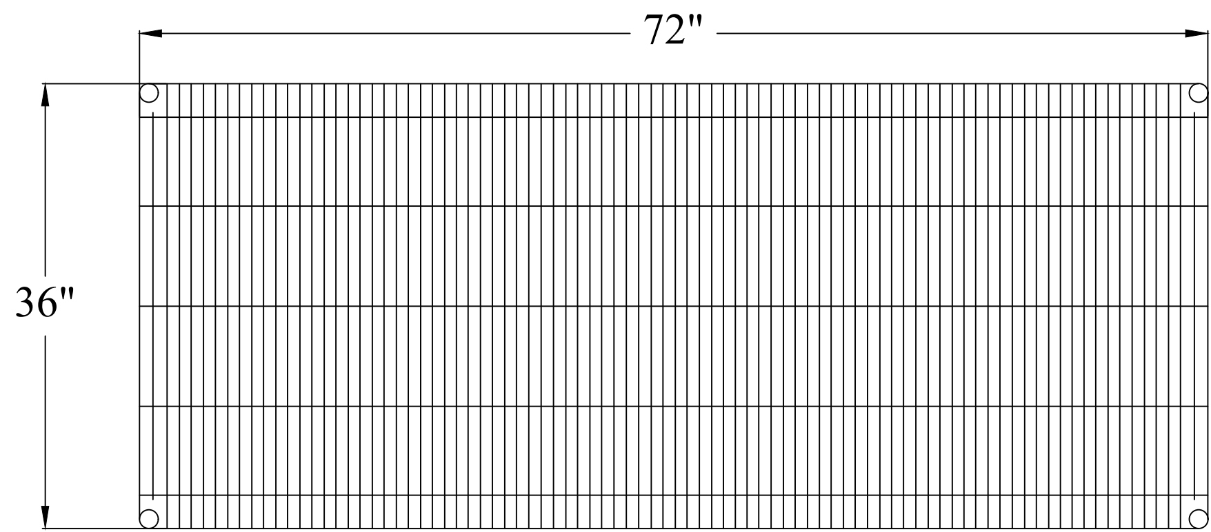
TOP VIEW
